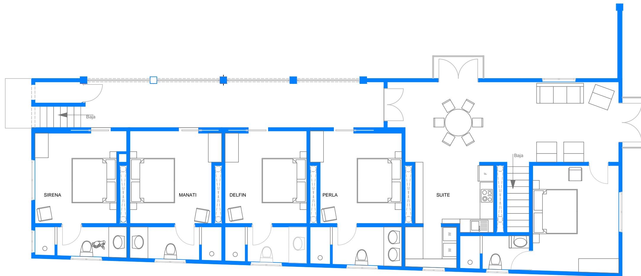
NEW CASITA FIRST FLOOR
