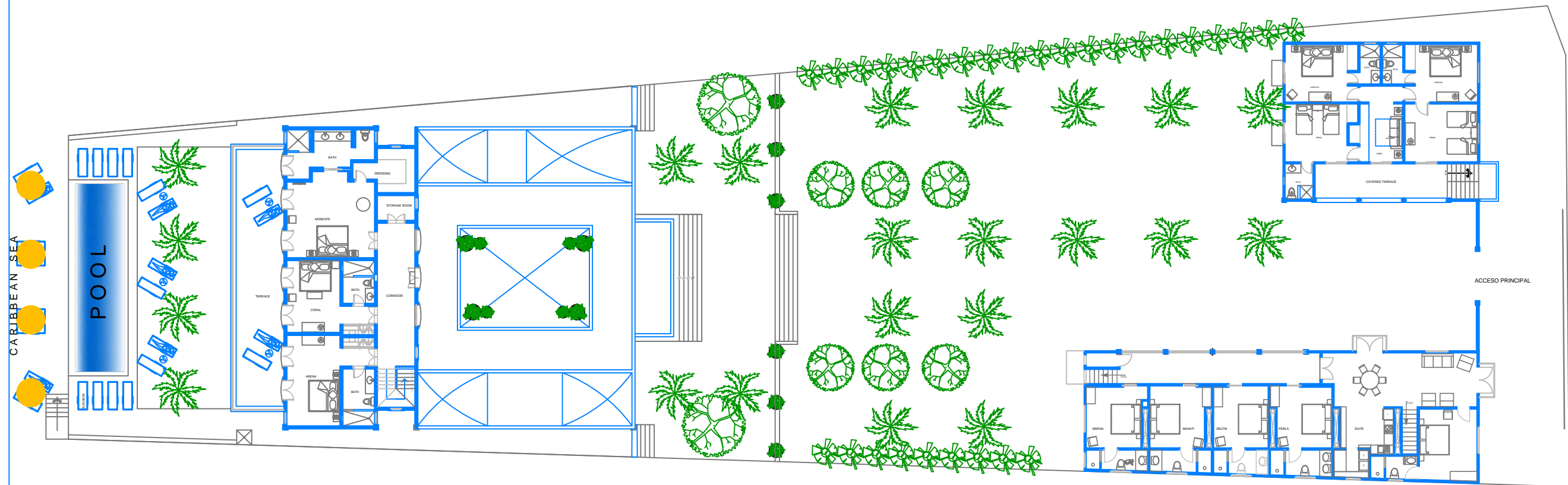
OVERALL FIRST FLOOR PLAN
